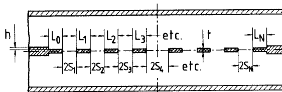
Fig. 1. Figure of Table I with correct designation of the slot lengths.
